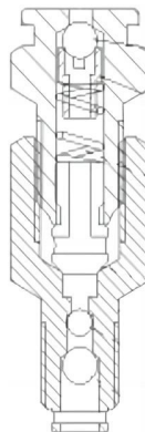
Lock Seal Fitting – Double Check
