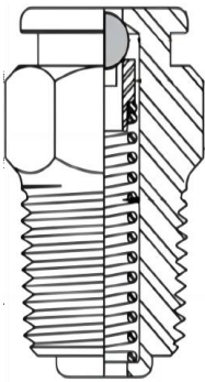
Gaint button head fitting-Single ball
