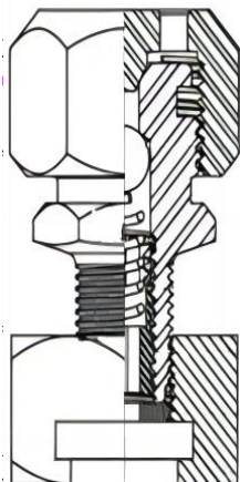
Leak locker fitting Gaint button head
