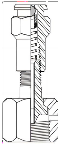
Lock Seal Fitting – Double Check
