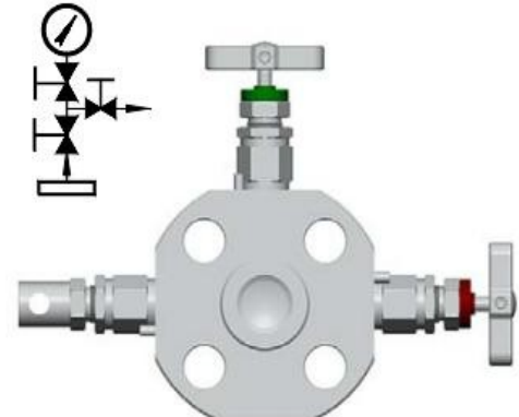
DBB series Block Block Bleed
