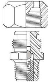
Lubrication (Sealant) Packing Injection Fitting 9/16" Autoclave Style
