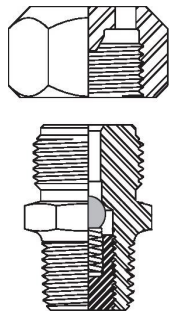
Free Flow Vented Cap Body Grease Fittings without Giant Button
